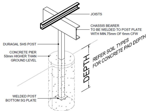
FOOTING DETAIL SUB-FLOOR POSTS
