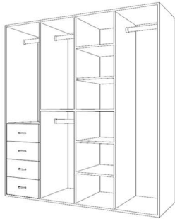
2 doors 1500 - 2400mm
