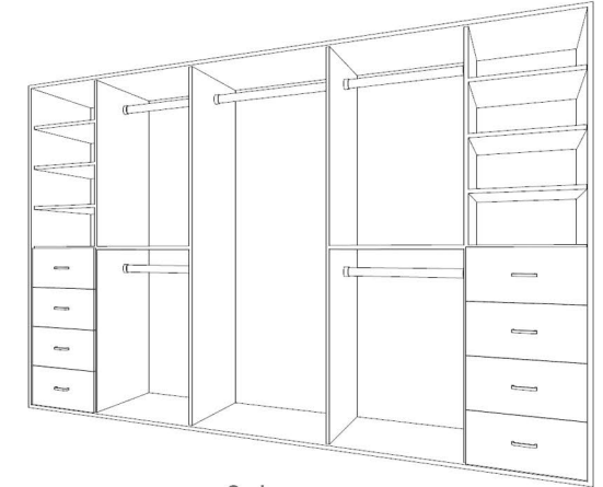
3 doors 2700 - 3600mm
